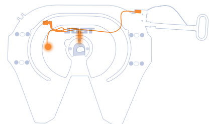
JSK 37 CZS/CWS Sensor Coupling
